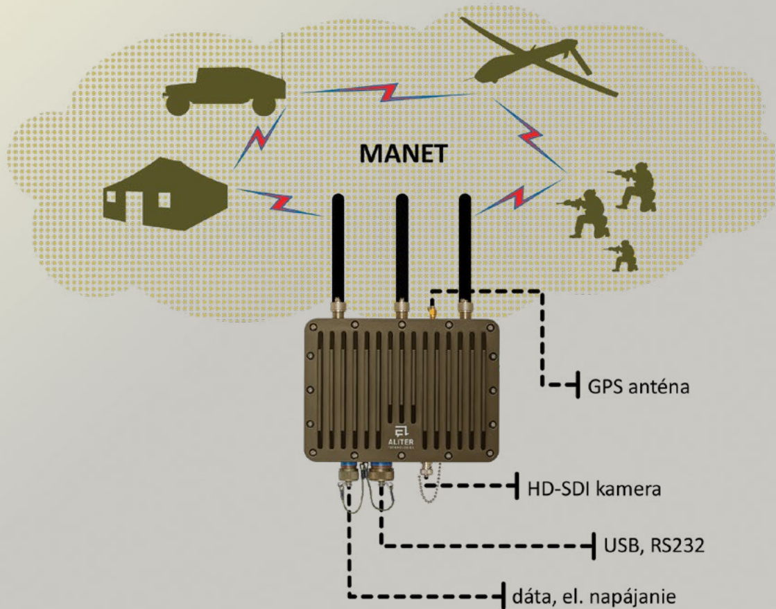
B2R (AT23703) - ROZHRANIA
